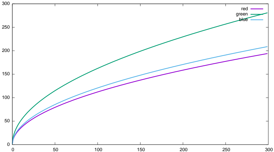
Conversion curves - Apple, iPhone 6s, 100 ISO (07012017144935)
