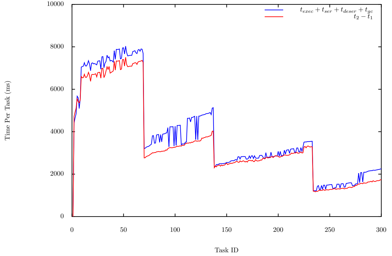
Figure 1: A comparison of time to complete tasks from measurements reported in the Spark event log. The difference in the reported launch and finish times, t_2 - t_1 , is compared to the sum of the elapsed times reported for: serialization, garbage collection, and execution components of each task.
