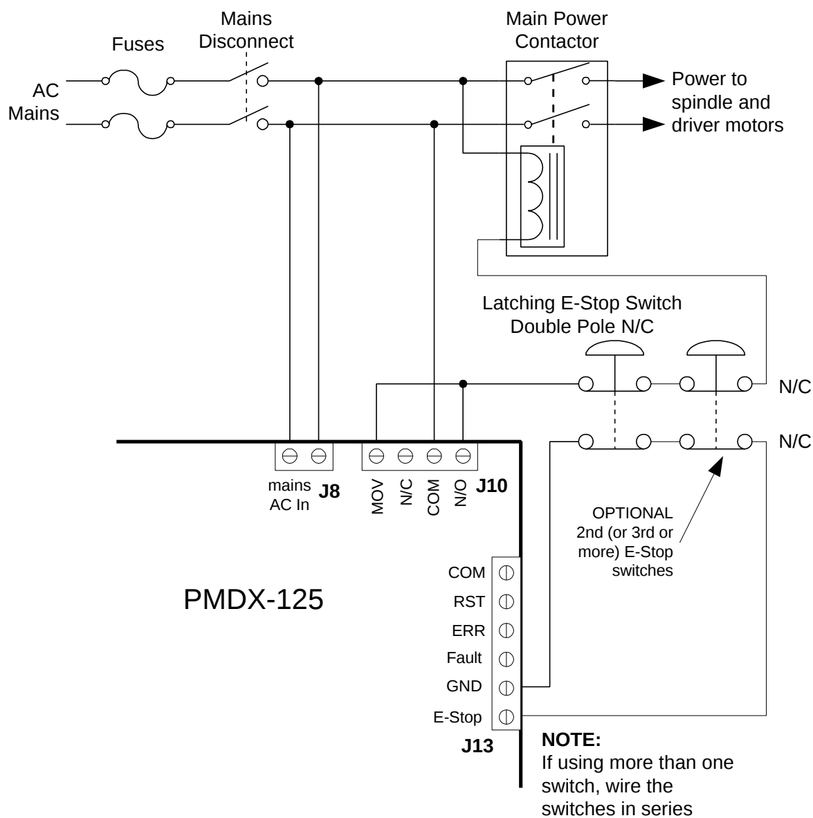
Figure 1 - Power Interrupt Circuit with Dual E-Stop Switch with two normally closed (N/C) set of contacts
