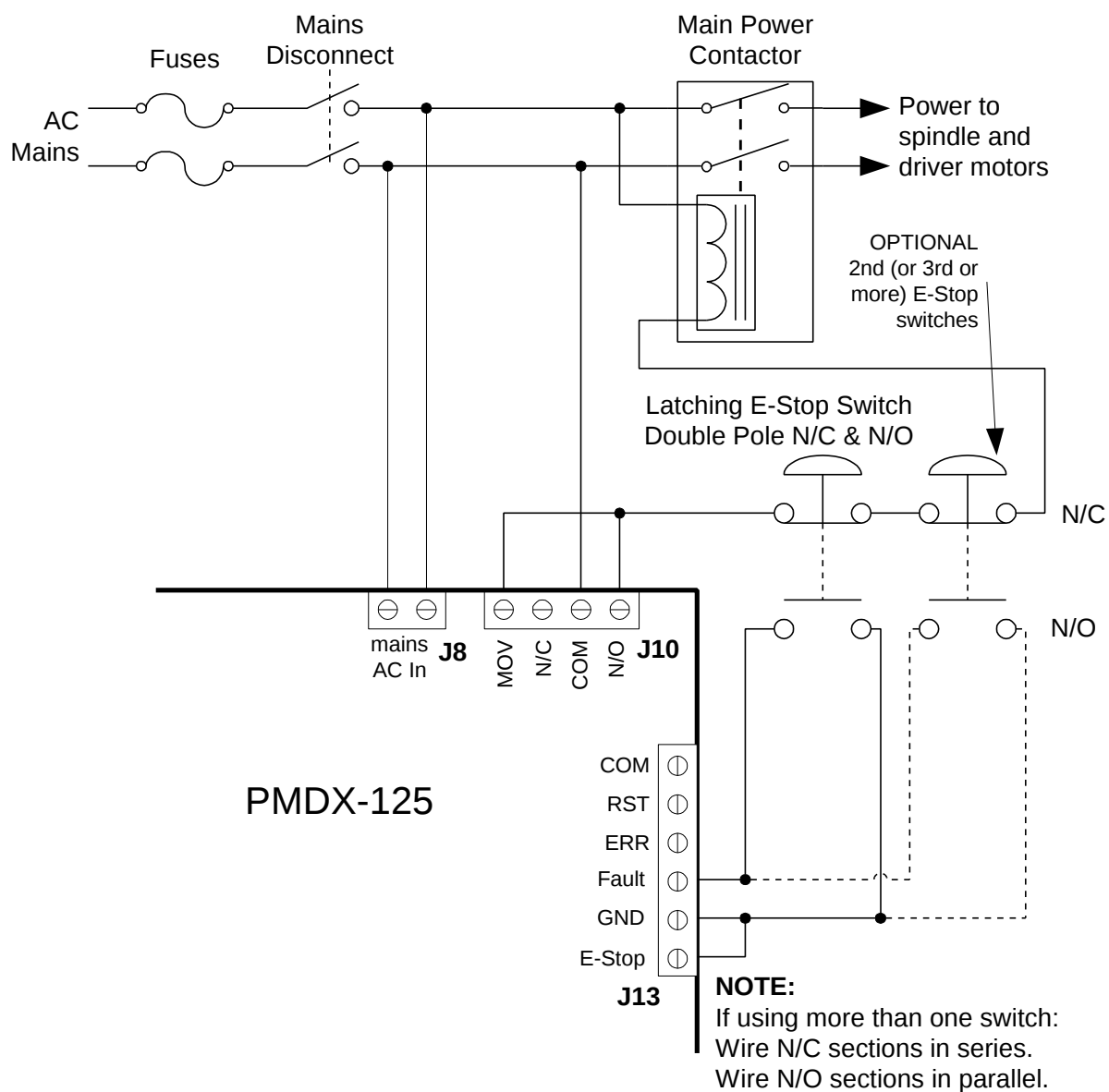
Figure 2 - Power Interrupt Circuit with Dual E-Stop Switch with one normally closed (N/C) and one normally open (N/O) set of contacts
