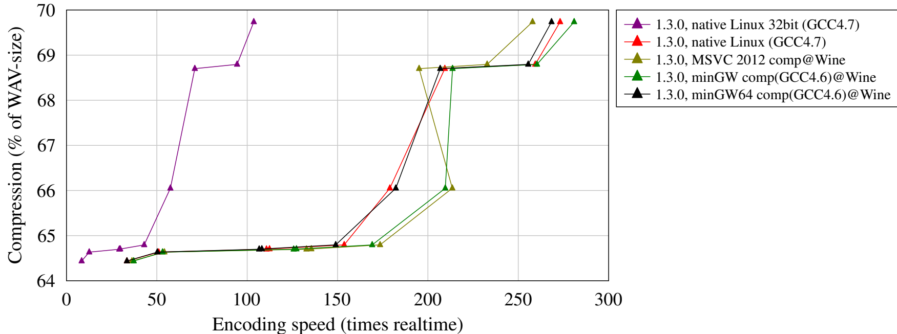
Encoding speed vs compression (30 Seconds to Mars - This Is War)
