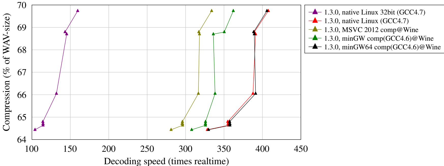
Decoding speed vs compression (30 Seconds to Mars - This Is War)
