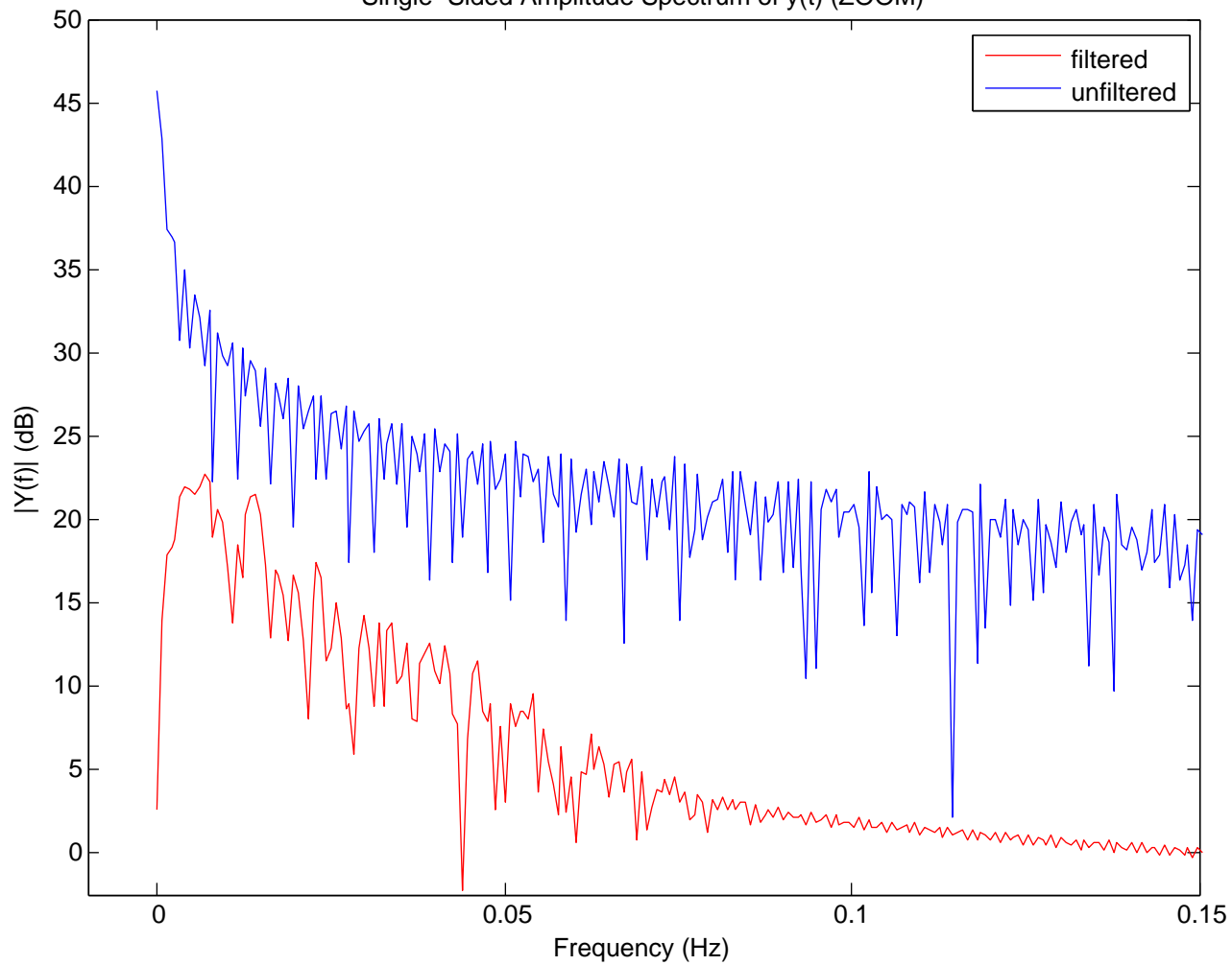
Single-Sided Amplitude Spectrum of y(t) (ZOOM)
