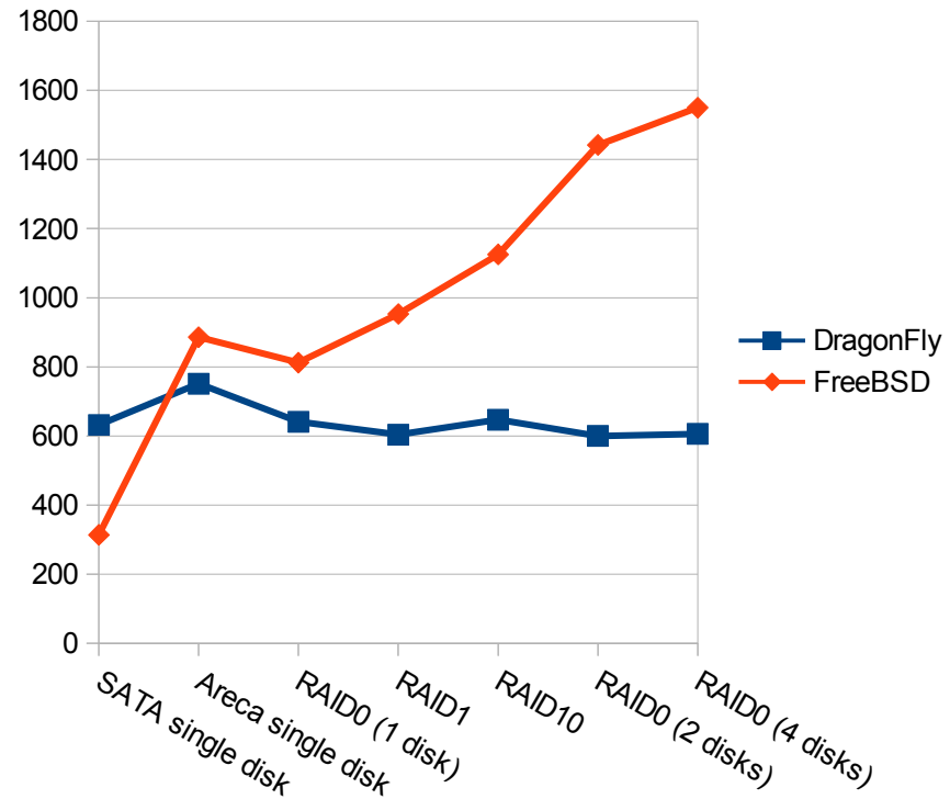
Blogbench writes
