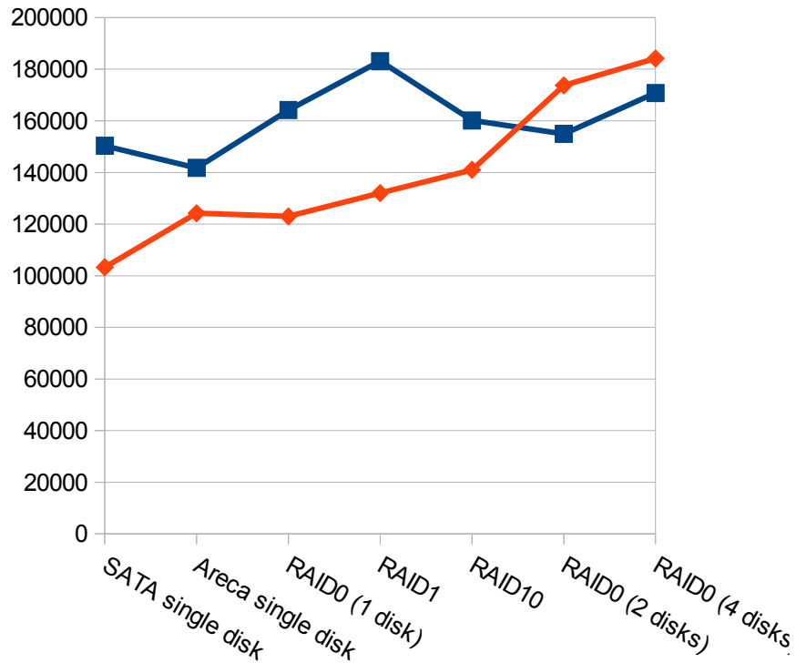
Blogbench reads
