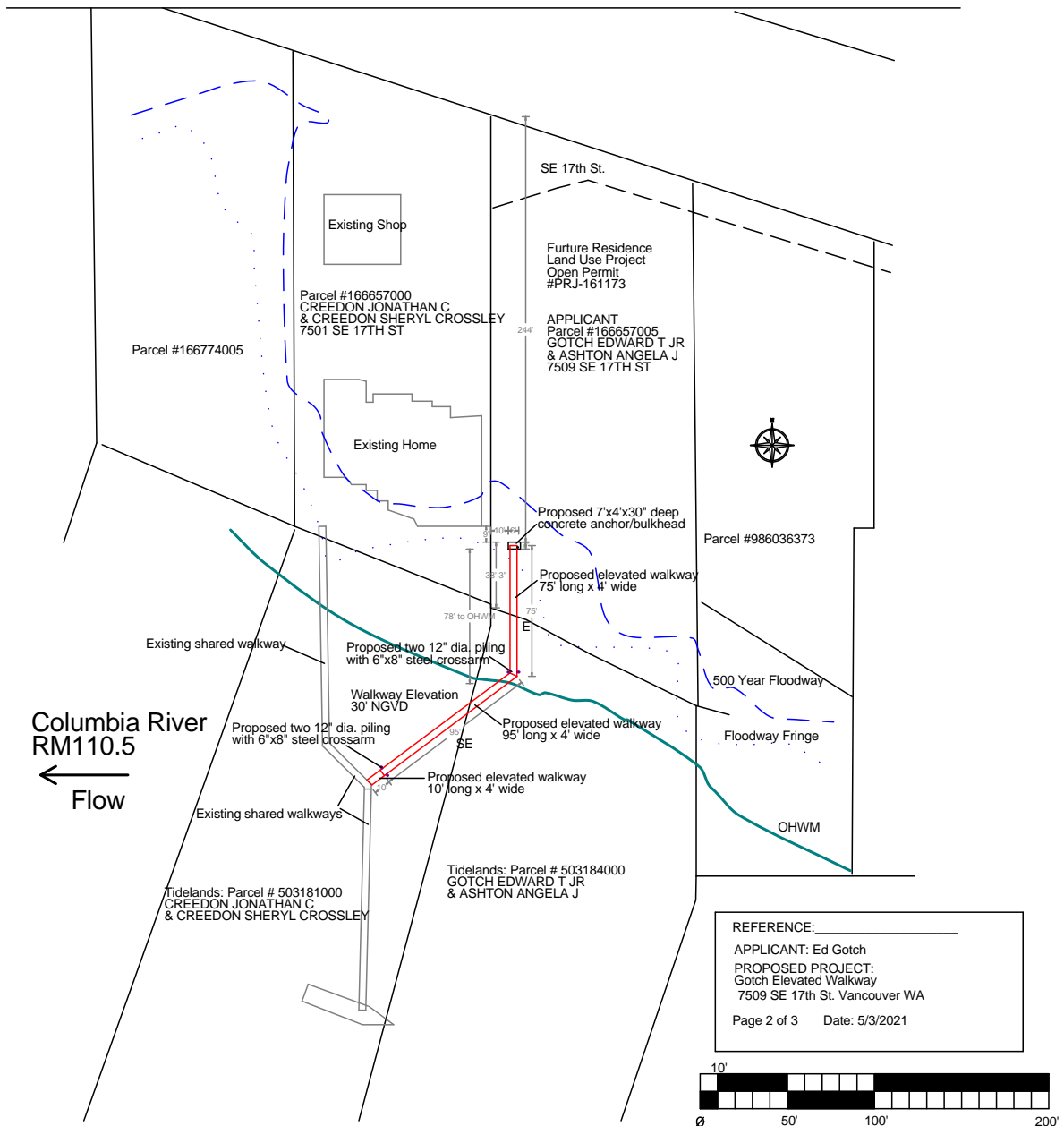
Figure 0.1: The elevated walkway project site plan.
