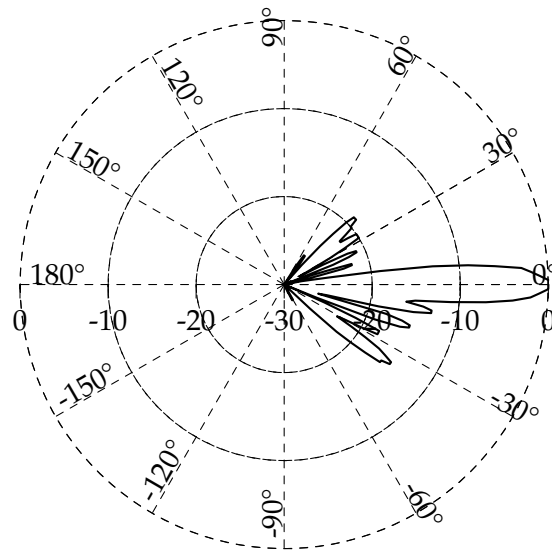
FIGURE 0.1 – A vertical antenna radiation pattern
